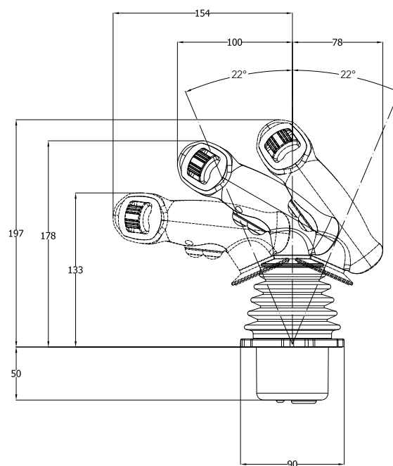
JHM base with HR type handle Complete code: JHM-L4C/NN-HR-0FP9-2P9/R000
