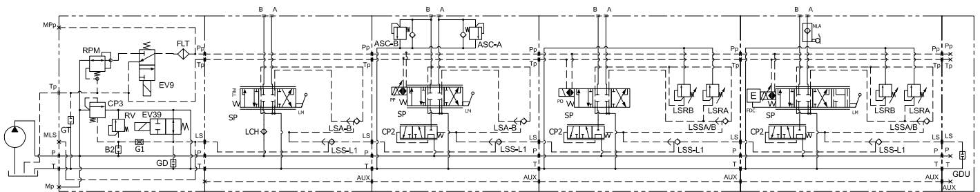
ELECTRO-HYDRAULIC SCHEMATIC
