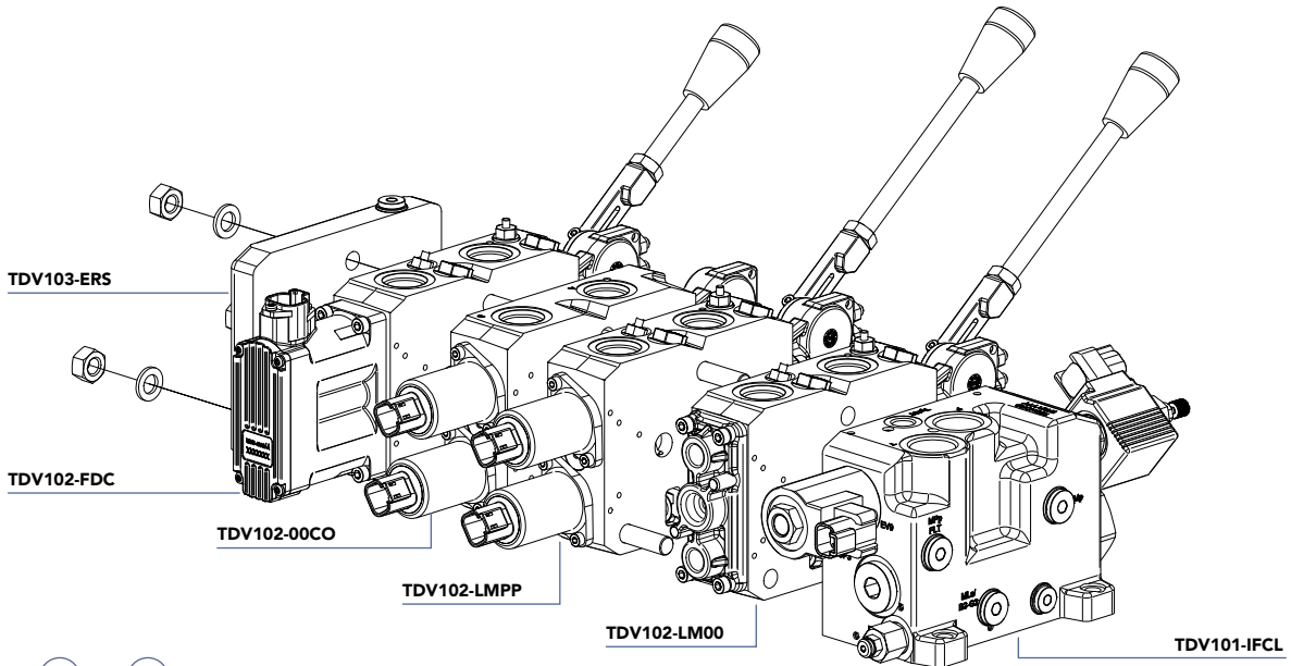
TDV101-IFCL/IVOL Inlet section for FIXED (FC) or VARIABLE (VO) displacement pump / LEFT HAND version
