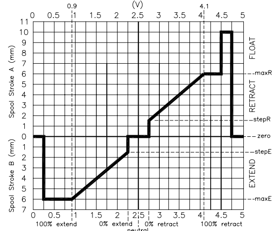
VALVE SPOOL STROKE (mm) VS. INPUT SIGNAL (Volt DC)
